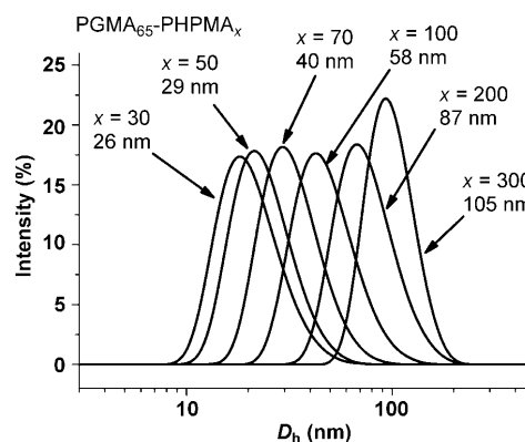
Figure 1. Dynamic light scattering particle size distributions obtained for a series of PGMA 65 –PHPMA x nanolatexes in which the PGMA block length is fixed and the PHPMA block length is systematically varied.
